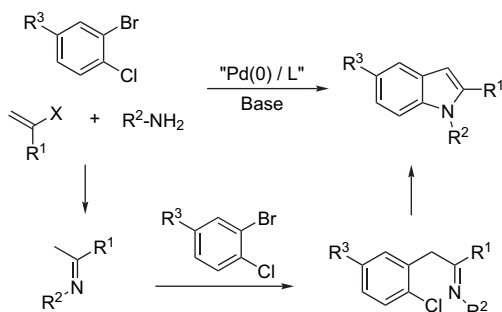
Scheme 2. Multicomponent synthesis of indoles promoted by a multifunctional Pd-catalyst.
